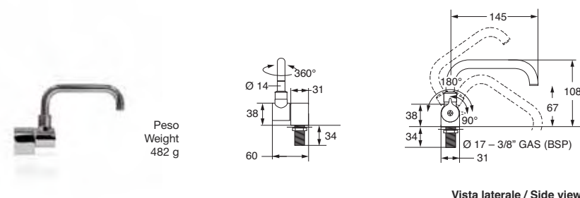
Vista laterale / Side view
