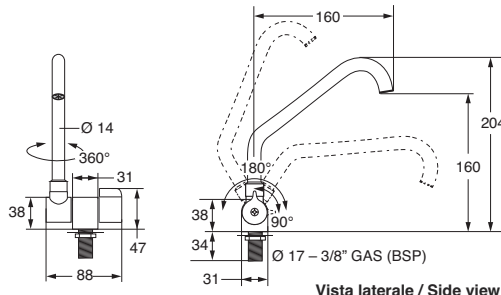
Vista laterale / Side view
