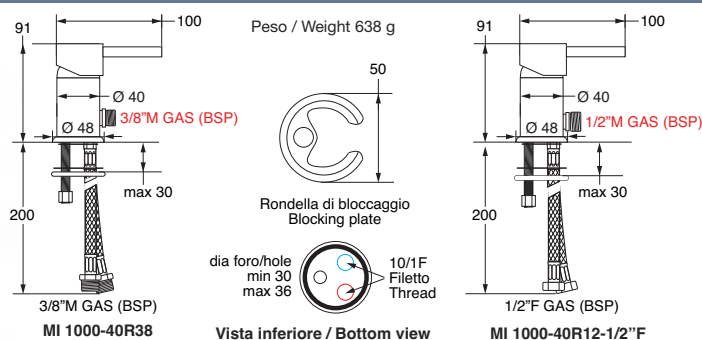
Maniglia / Handle SIMPLY
