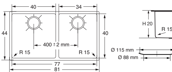
LV 40.40.34.20-C/15T/WD > SOTTOPIANO / UNDER SURFACE
