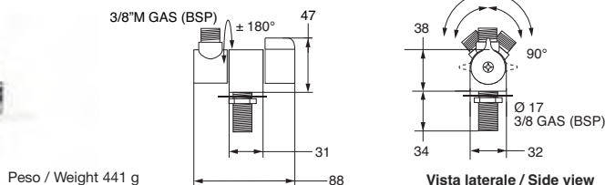
Maniglia / Handle MISTER
