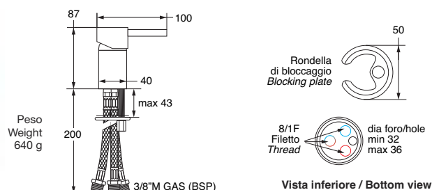
Maniglia / Handle SIMPLY
