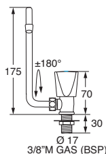
Vista laterale / Side view
