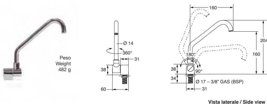
Vista laterale / Side view
