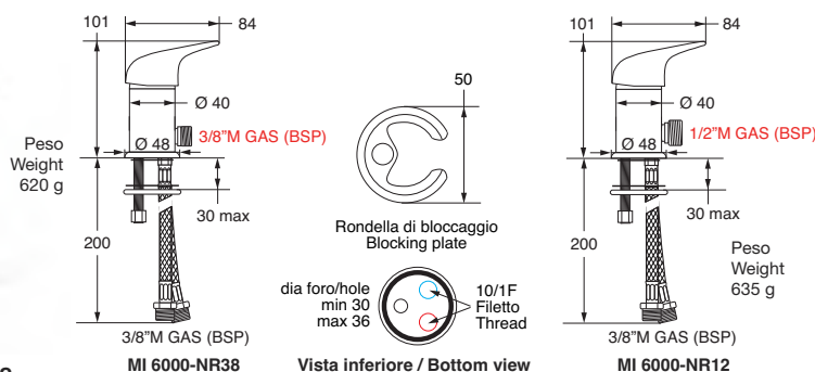
Maniglia / Handle KIMMY
